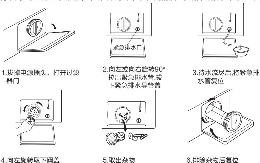
4.向左旋转取下阀盖
